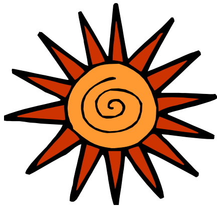
15. Heat waves
